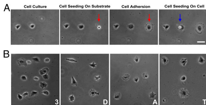
Fig. 6. Printing living cells with 3D acoustic tweezers. (A) Single-cell printing. After previously deposited 3T3 cells were attached to the substrate, another single cell was picked up, transported, and dropped at the desired location on the substrate (indicated by red arrow) or on top of another cell (indicated by blue arrow). The single cell adhered and spread along the surface. (B) Formation of arbitrary cell culture patterns forming a “3” “D” “A” and “T” by printing of single HeLa S3 cells via 3D acoustic tweezers. (Scale bar: 20 \mu\text{m} .)
