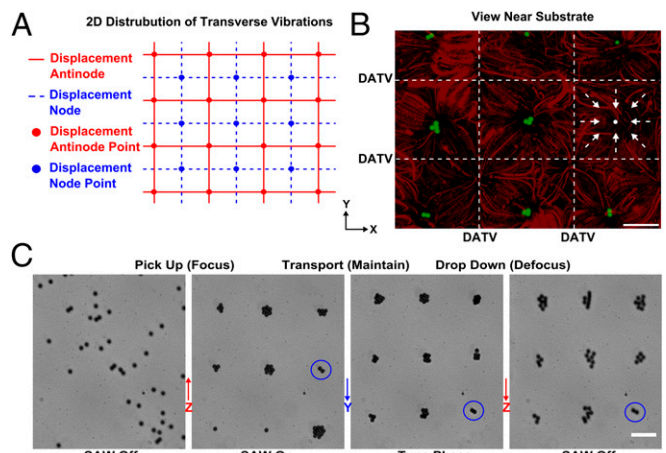
Fig. 5. Three-dimensional acoustic manipulation. (A) Illustration of the 2D distribution of transverse vibrations on the substrate. Blue lines represent displacement nodes of transverse vibrations that have minimal vibration amplitudes; red lines represent displacement antinodes. (B) Superimposed images of 3D trapping and streaming patterns; 10\text{-}\mu\text{m} green fluorescent polystyrene particles were trapped into a suspended array of single dots, and 1\text{-}\mu\text{m} red fluorescent polystyrene particles tracked the motion of the acoustic streaming vortex (the arrows indicate the direction of the streaming near the substrate surface). (C) The image sequence shows the 3D trapping and manipulation of particles with a stable array configuration. A trapping node (blue circle) can levitate particles along z axis (moving into focus) and pushing particles together, transporting them along y axis and dropping them back toward the substrate (moving out of focus). (Scale bar: 100\text{ }\mu\text{m} .)
